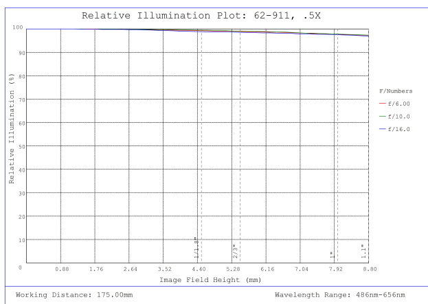
#62-911, 0.5X Cobalt TL Telecentric Lens, Relative Illumination Plot
