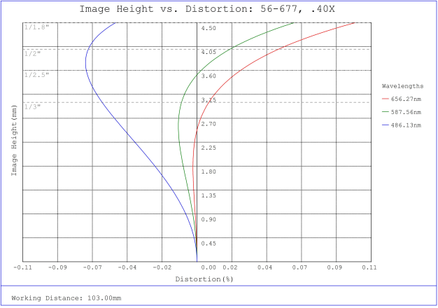
#56-677, 0.40X SilverTL™ Telecentric Lens, Distortion Plot
