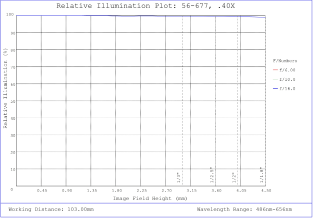
#56-677, 0.40X SilverTL™ Telecentric Lens, Relative Illumination Plot
