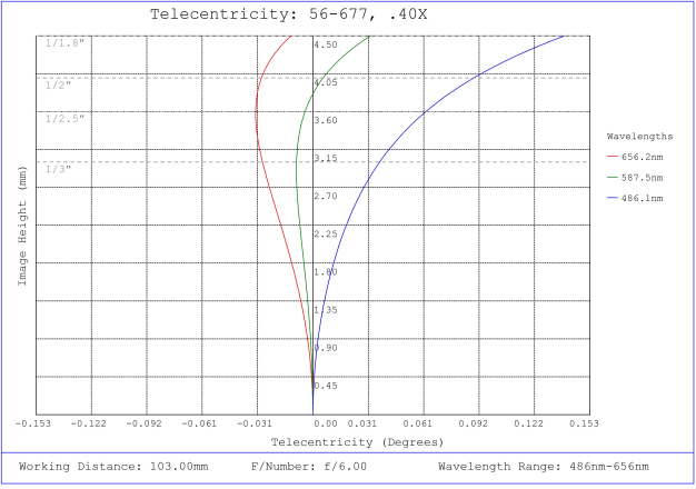
#56-677, 0.40X SilverTL™ Telecentric Lens, Telecentricity Plot
