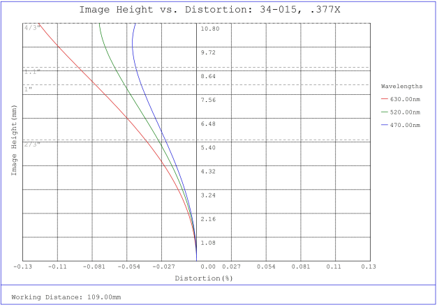
#34-015, 0.377X, 4/3" C-Mount TitanTL® Telecentric Lens, Distortion Plot
