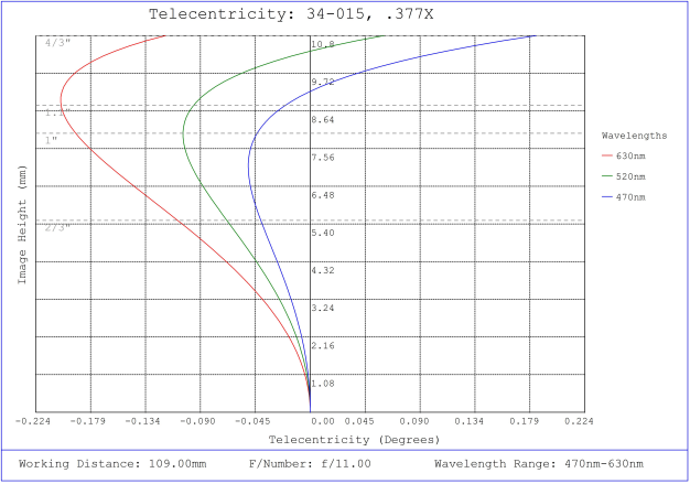
#34-015, 0.377X, 4/3" C-Mount TitanTL® Telecentric Lens, Telecentricity Plot
