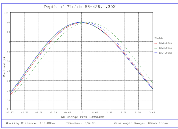
#58-428, 0.30X SilverTL™ Telecentric Lens, Depth of Field Plot, 139mm Working Distance, f6
