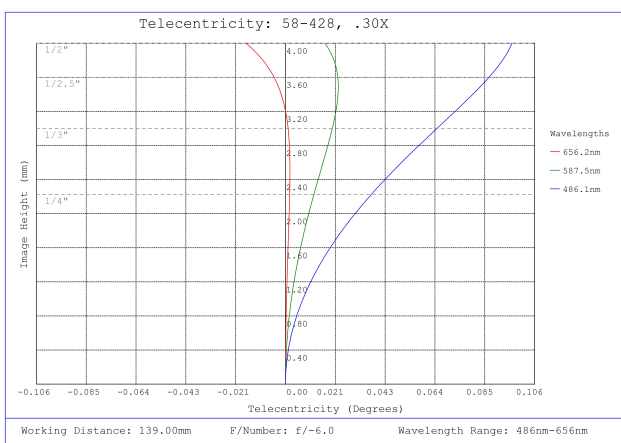
#58-428, 0.30X SilverTL™ Telecentric Lens, Telecentricity Plot
