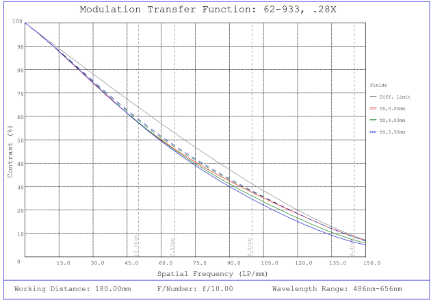
#62-933, 0.28X, 2/3" C-Mount PlatinumTL™ Telecentric Lens, Modulated Transfer Function (MTF) Plot, 180mm Working Distance, f10
