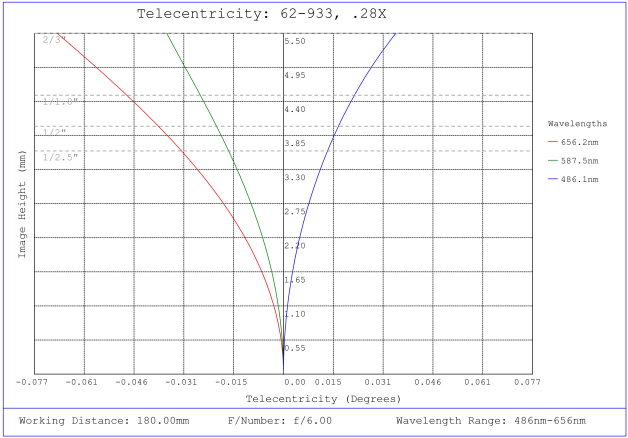
#62-933, 0.28X, 2/3" C-Mount PlatinumTL™ Telecentric Lens, Telecentricity Plot
