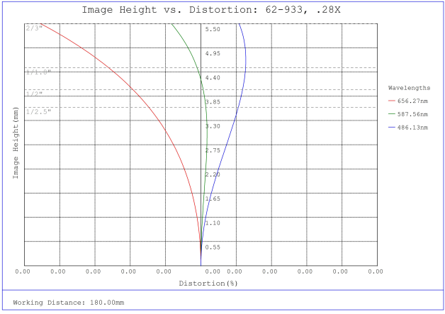
#62-933, 0.28X, 2/3" C-Mount PlatinumTL™ Telecentric Lens, Distortion Plot
