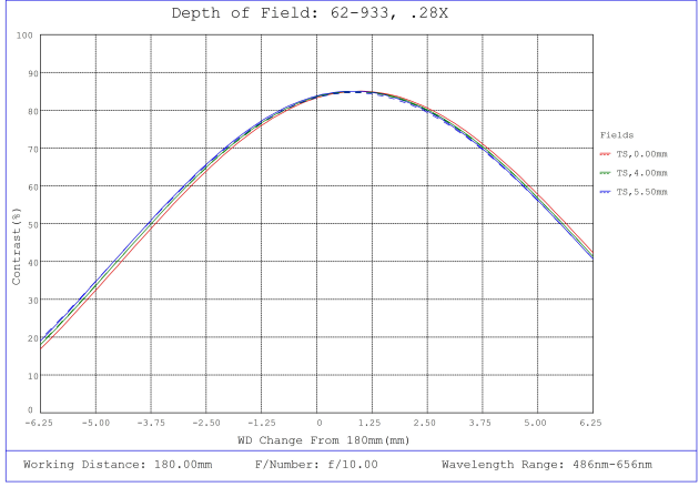
#62-933, 0.28X, 2/3" C-Mount PlatinumTL™ Telecentric Lens, Depth of Field Plot, 180mm Working Distance, f10
