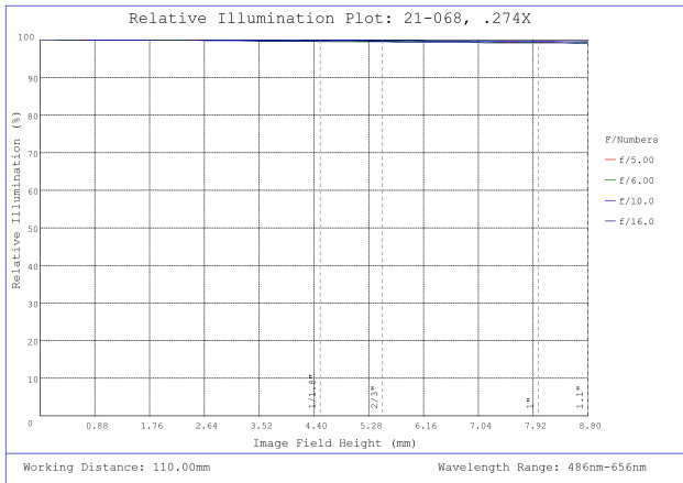
#21-068, 0.274X Cobalt TL Telecentric Lens, Relative Illumination Plot
