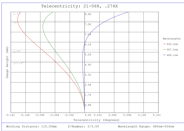
#21-068, 0.274X Cobalt TL Telecentric Lens, Telecentricity Plot
