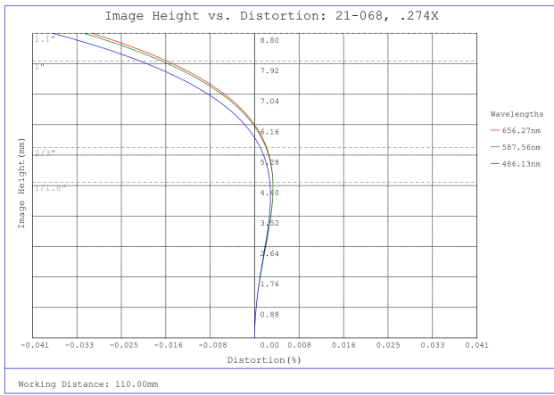
#21-068, 0.274X CobaltTL Telecentric Lens, Distortion Plot
