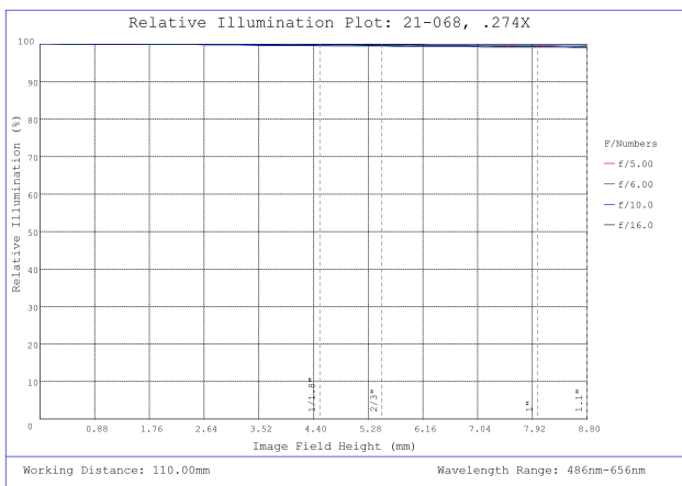
#21-068, 0.274X CobaltTL Telecentric Lens, Relative Illumination Plot
