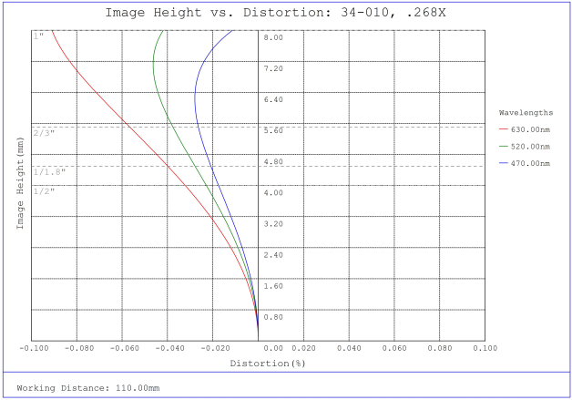
#34-010, 0.268X, 1" C-Mount TitanTL® Telecentric Lens, Distortion Plot
