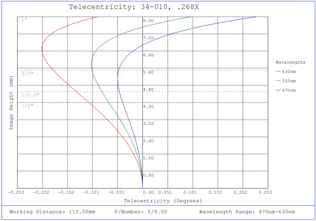
#34-010, 0.268X, 1" C-Mount TitanTL® Telecentric Lens, Telecentricity Plot
