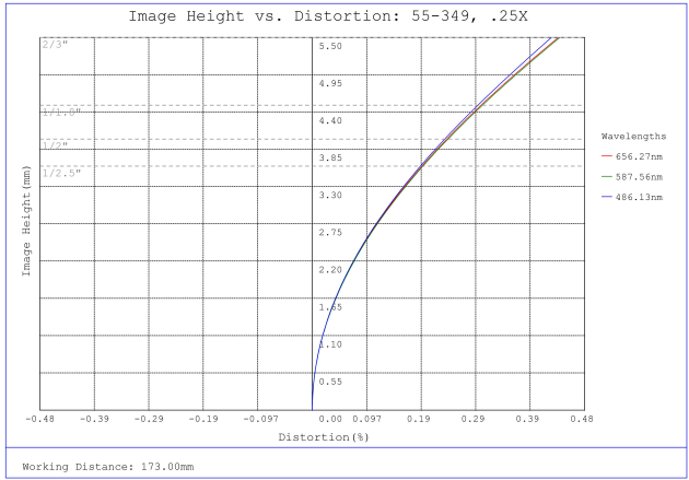
#55-349, 0.25X 2/3" GoldTL™ Telecentric Lens, Distortion Plot
