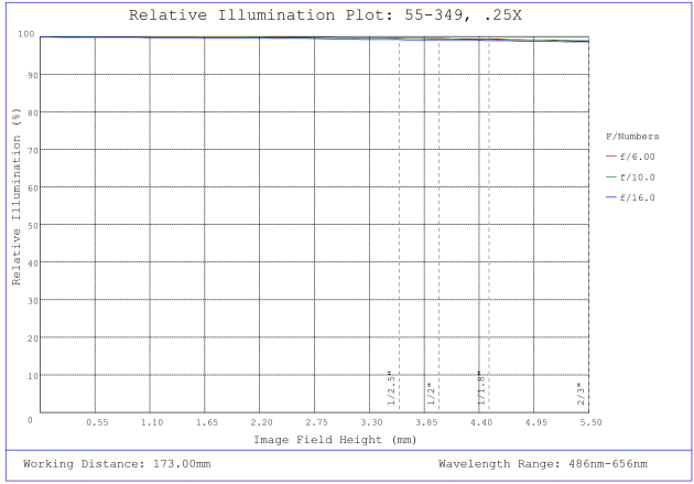
#55-349, 0.25X 2/3" GoldTL™ Telecentric Lens, Relative Illumination Plot
