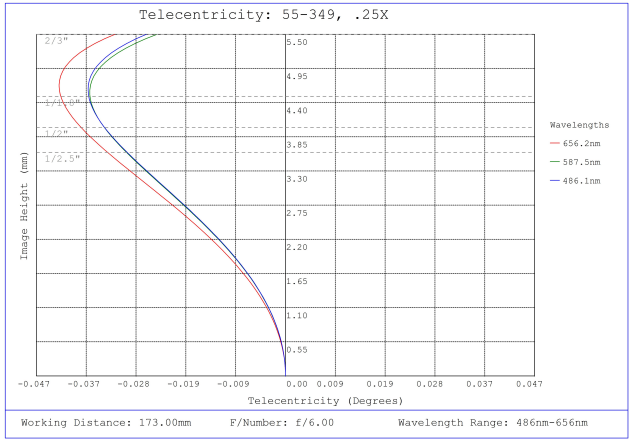
#55-349, 0.25X 2/3" GoldTL™ Telecentric Lens, Telecentricity Plot
