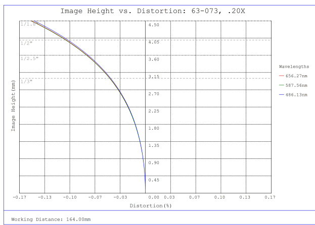
#63-073, 0.20X SilverTL™ Telecentric Lens, Distortion Plot
