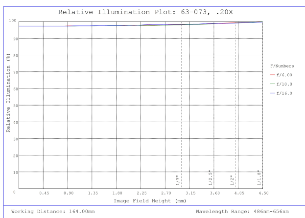
#63-073, 0.20X SilverTL™ Telecentric Lens, Relative Illumination Plot
