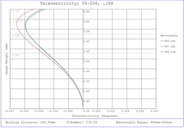
#58-258, 0.18X ½" GoldTL™ Telecentric Lens, Telecentricity Plot
