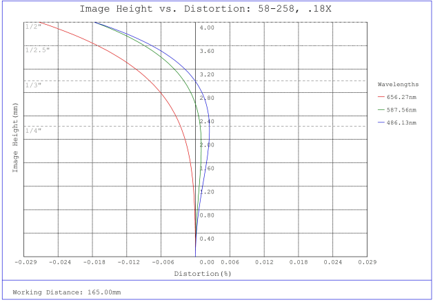
#58-258, 0.18X ½" GoldTL™ Telecentric Lens, Distortion Plot
