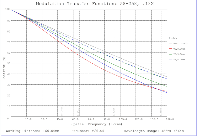
#58-258, 0.18X ½" GoldTL™ Telecentric Lens, Modulated Transfer Function (MTF) Plot, 165mm Working Distance, f6
