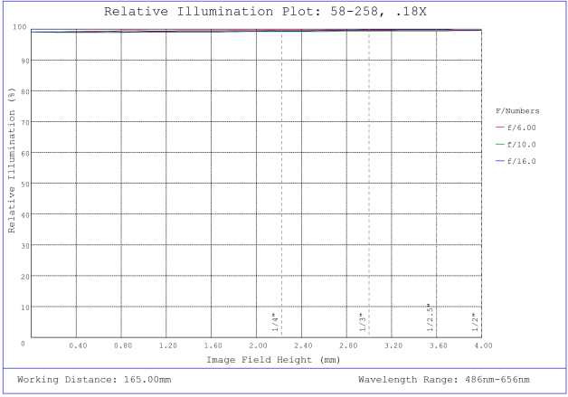
#58-258, 0.18X ½" GoldTL™ Telecentric Lens, Relative Illumination Plot
