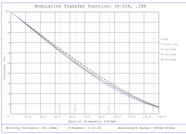
#58-258, 0.18X 1/2" GoldTL™ Telecentric Lens, Modulated Transfer Function (MTF) Plot, 165mm Working Distance, f10
