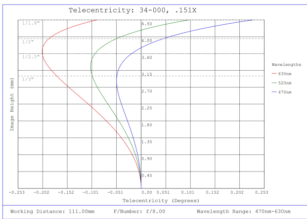
#34-000, 0.151X, 1/1.8" C-Mount TitanTL® Telecentric Lens, Telecentricity Plot
