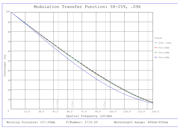
#58-259, 0.09X 1/2" GoldTL™ Telecentric Lens, Modulated Transfer Function (MTF) Plot, 157mm Working Distance, f10
