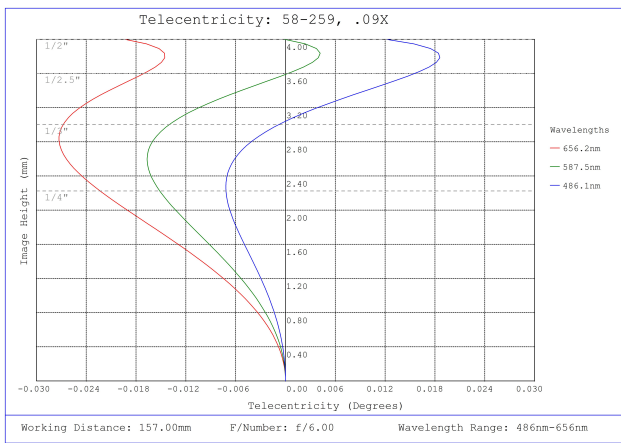
#58-259, 0.09X 1/2" GoldTL™ Telecentric Lens, Telecentricity Plot
