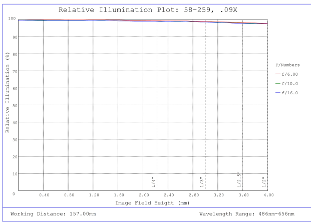
#58-259, 0.09X 1/2" GoldTL™ Telecentric Lens, Relative Illumination Plot
