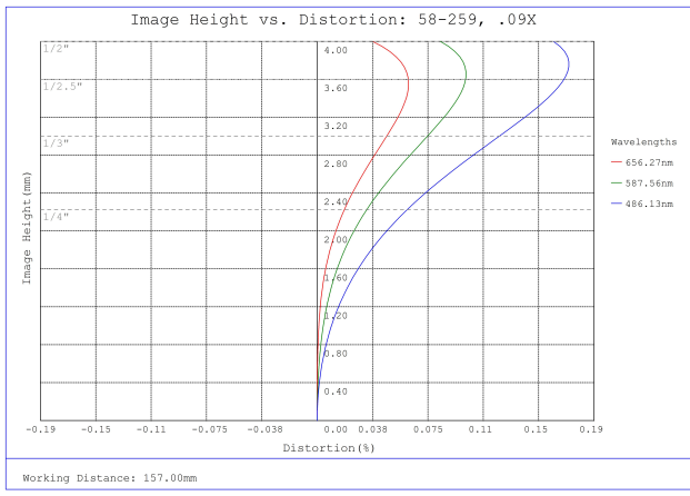
#58-259, 0.09X 1/2" GoldTL™ Telecentric Lens, Distortion Plot
