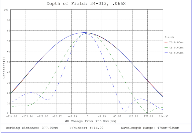
#34-013, 0.066X, 1" C-Mount TitanTL® Telecentric Lens, Depth of Field Plot, 377mm Working Distance, f16
