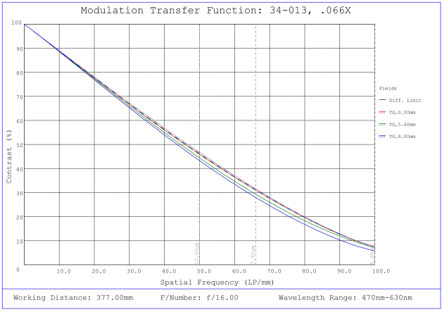
#34-013, 0.066X, 1" C-Mount TitanTL® Telecentric Lens, Modulated Transfer Function (MTF) Plot, 377mm Working Distance, f16
