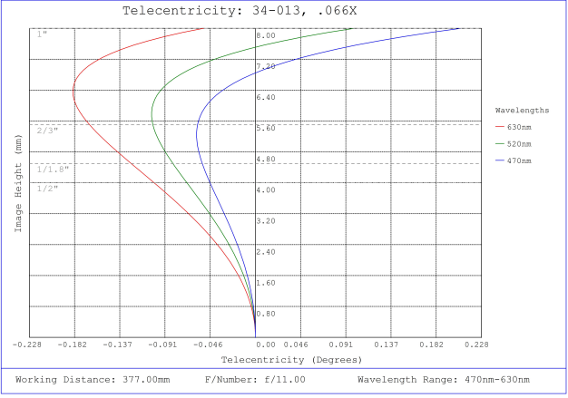
#34-013, 0.066X, 1" C-Mount TitanTL® Telecentric Lens, Telecentricity Plot
