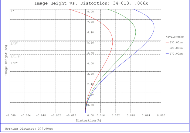
#34-013, 0.066X, 1" C-Mount TitanTL® Telecentric Lens, Distortion Plot
