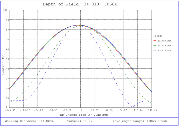
#34-013, 0.066X, 1" C-Mount TitanTL® Telecentric Lens, Depth of Field Plot, 377mm Working Distance, f11
