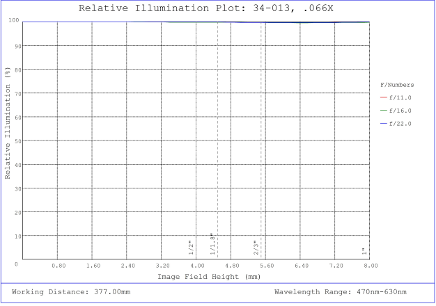
#34-013, 0.066X, 1" C-Mount TitanTL® Telecentric Lens, Relative Illumination Plot
