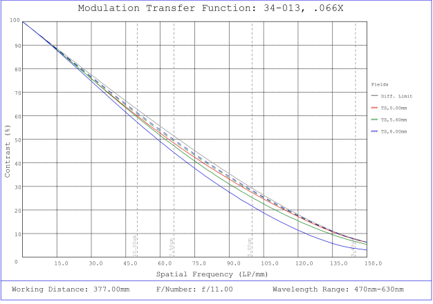
#34-013, 0.066X, 1" C-Mount TitanTL® Telecentric Lens, Modulated Transfer Function (MTF) Plot, 377mm Working Distance, f11
