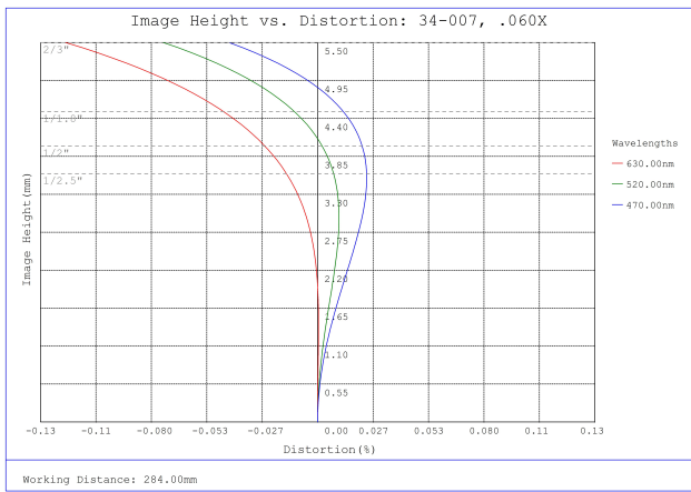
#34-007, 0.060X, 2/3" C-Mount TitanTL® Telecentric Lens, Distortion Plot
