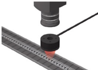
Workpiece image
