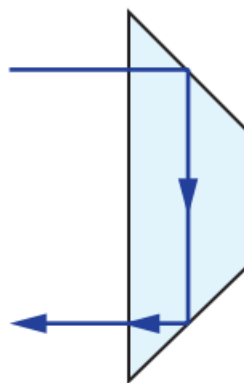
Aluminum Coated Dove Prism Ray Path
