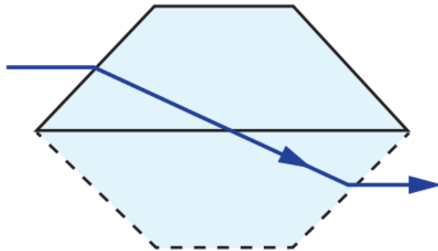
Dove Prisms Tunnel Diagram
