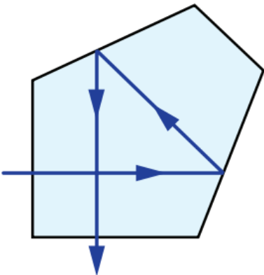
Penta Prism Ray Path
