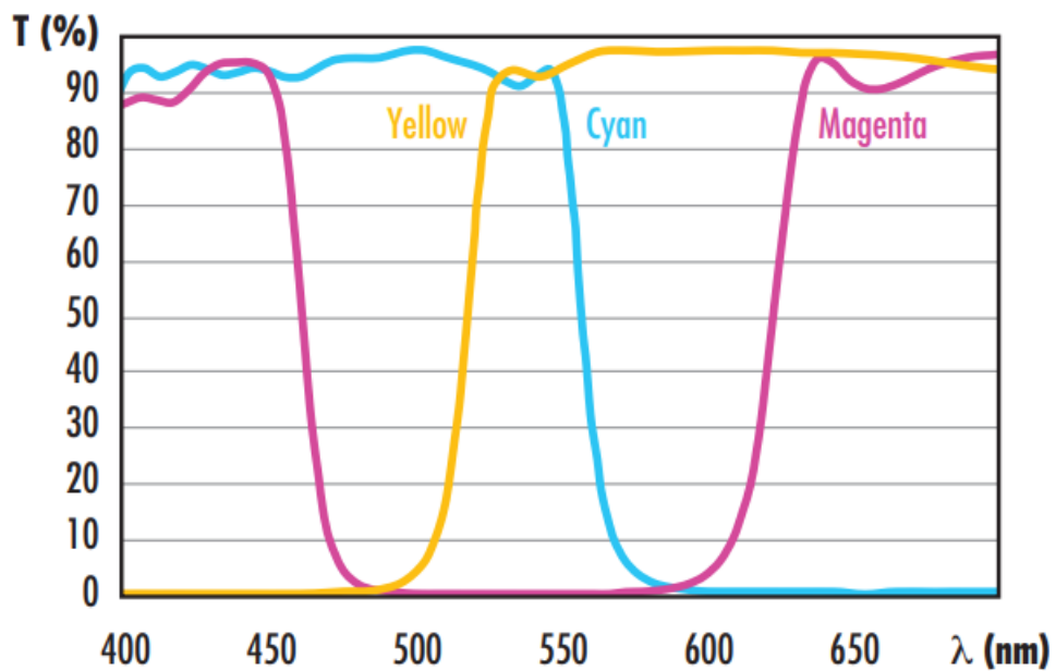
Subtractive Filters Typical Transmittance Curves
