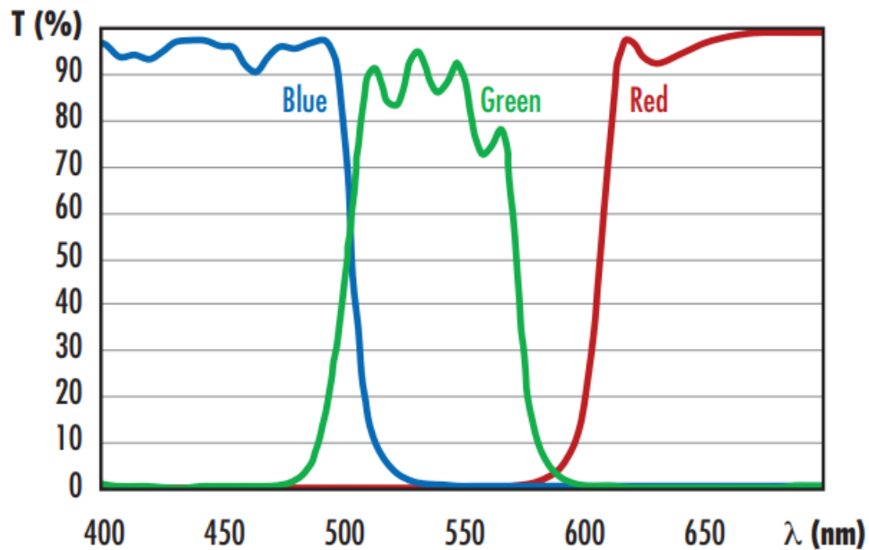
Additive Filters Typical Transmittance Curves
