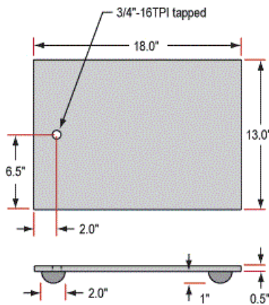
#54-262 Breadboard Adapter
