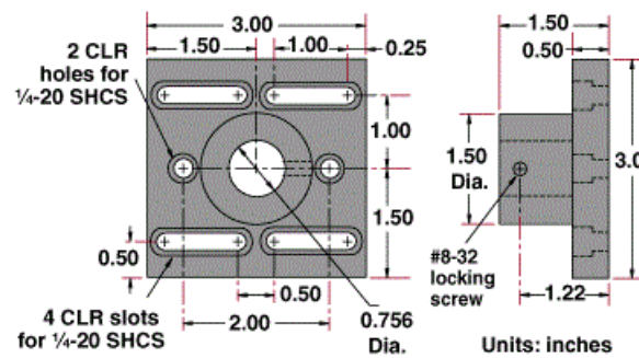
#54-262 Breadboard Adapter
