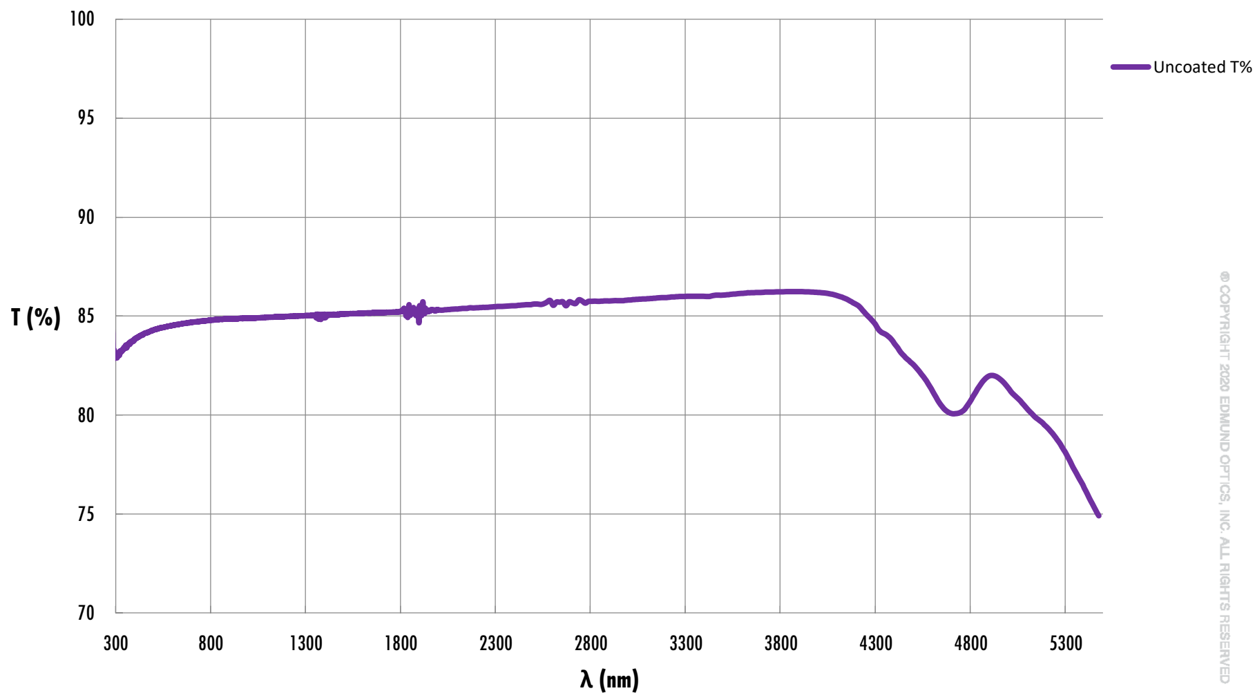
Coating Specification: Uncoated Theoretical Transmission Curve
