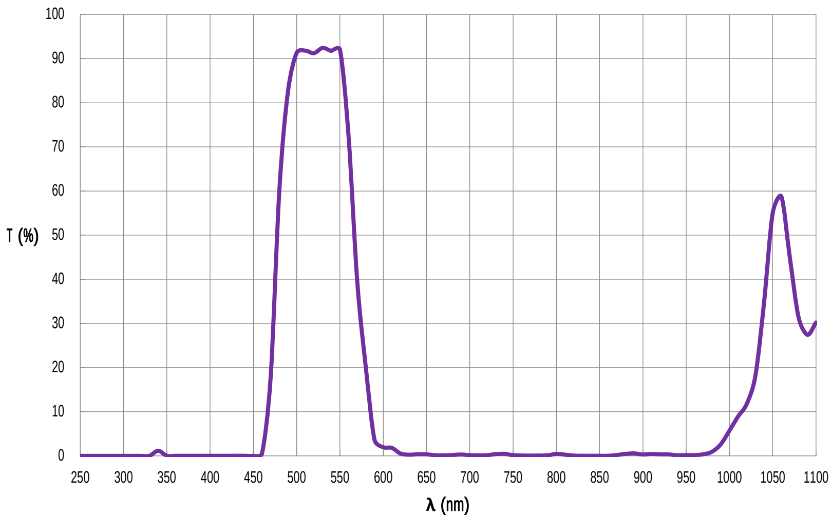
Cyan Machine Vision Bandpass Filter, 505nm FOR REFERENCE ONLY
