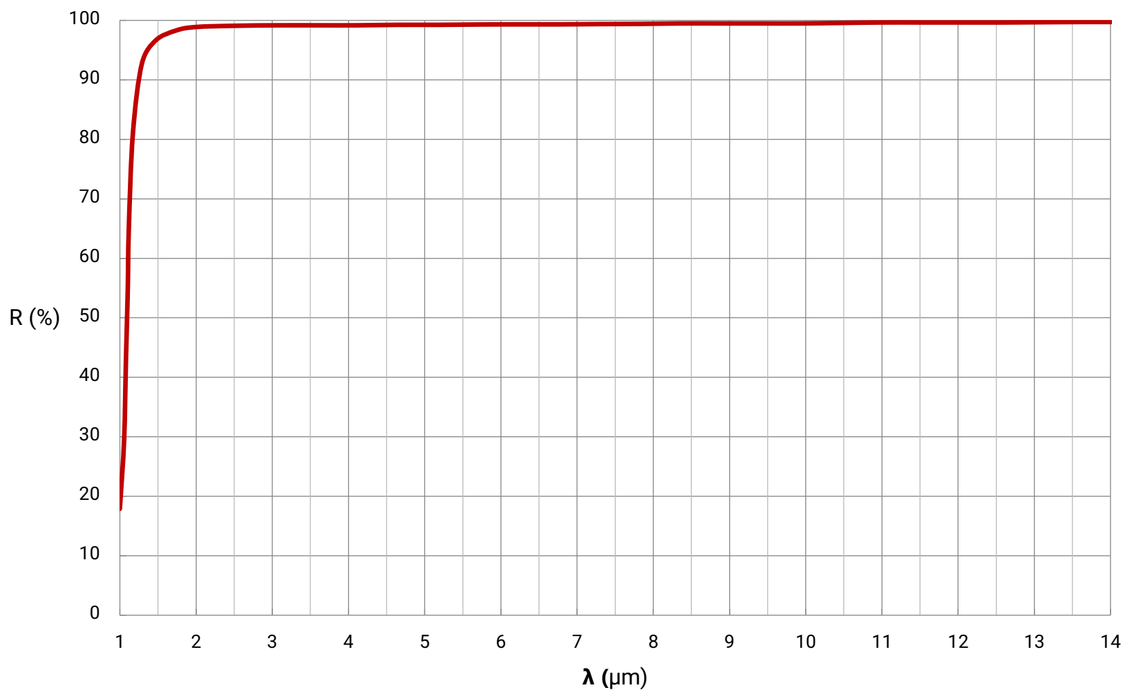
ISP Optics Protected Gold Coating Typical Reflectance Curve
