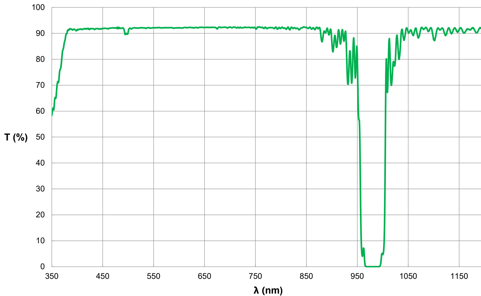
Everix Ultra-Thin OD 4 Notch Filter, 980nm, 12.5mm Diameter FOR REFERENCE ONLY
