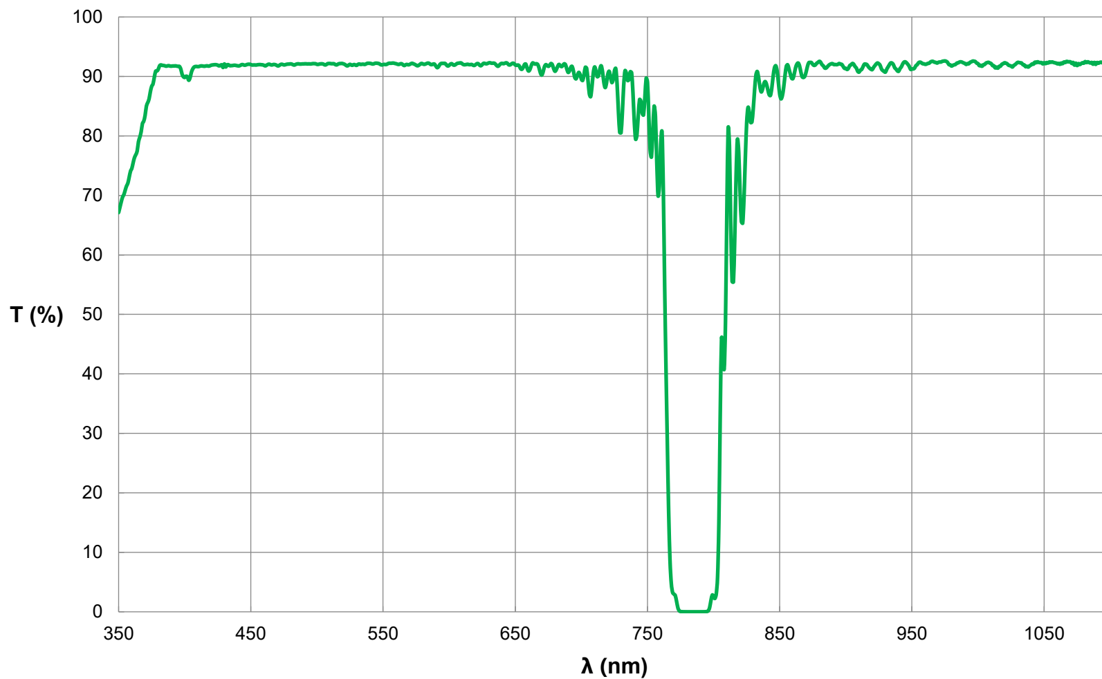
Everix Ultra-Thin OD 4 Notch Filter, 785nm, 12.5mm Diameter FOR REFERENCE ONLY
