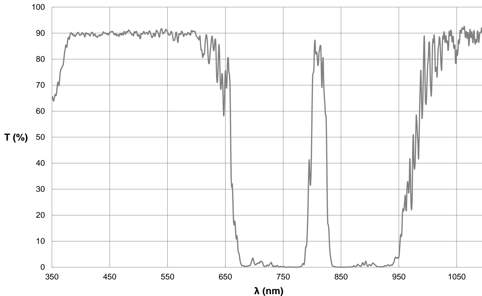
Everix Ultra-Thin Bandpass Filter, 810nm, OD 2.0 FOR REFERENCE ONLY
