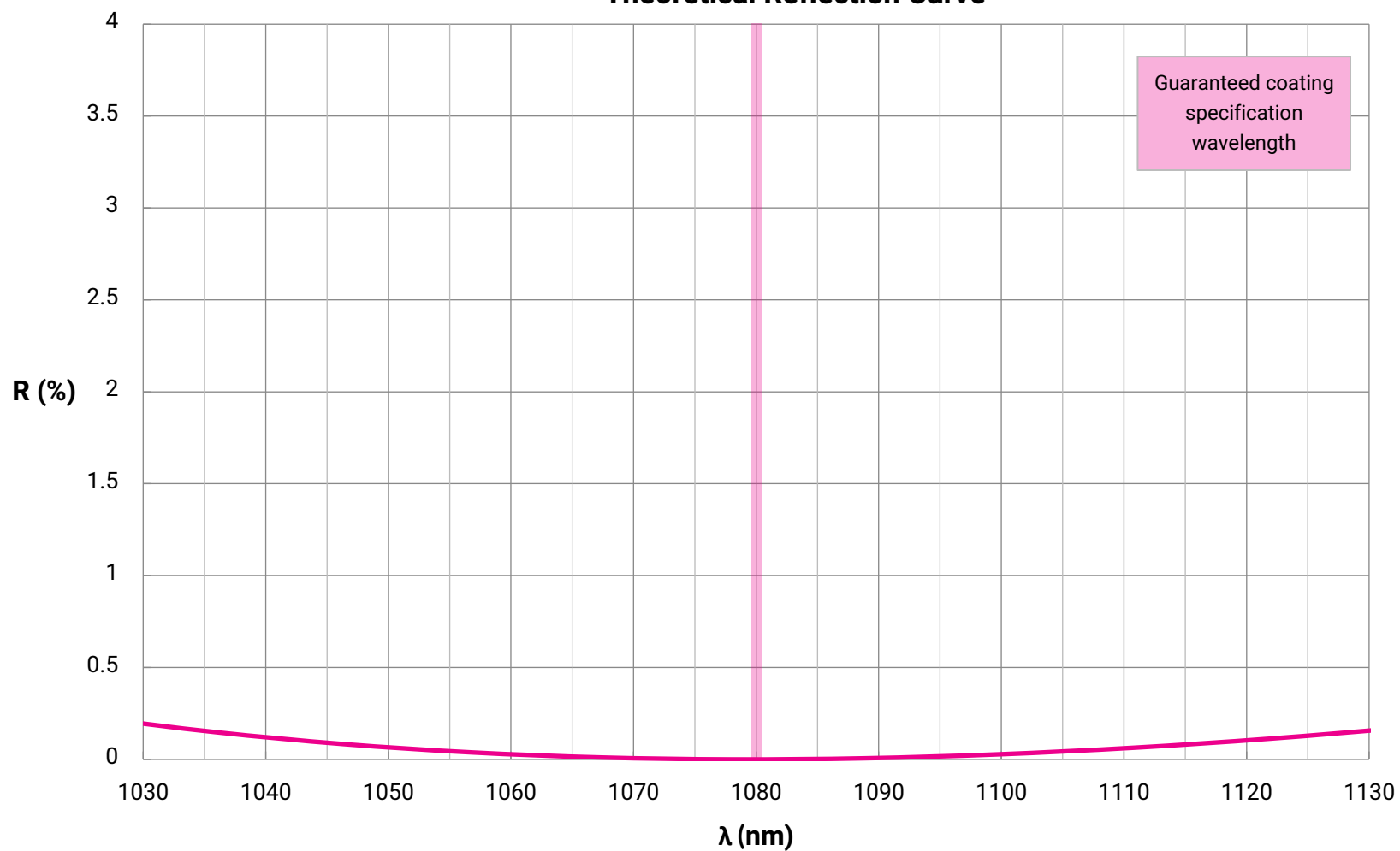
Theoretical Reflection Curve
