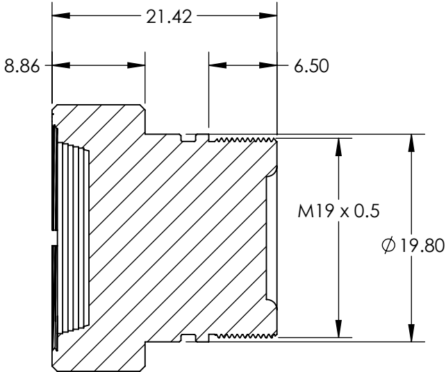
SECTION L-L
