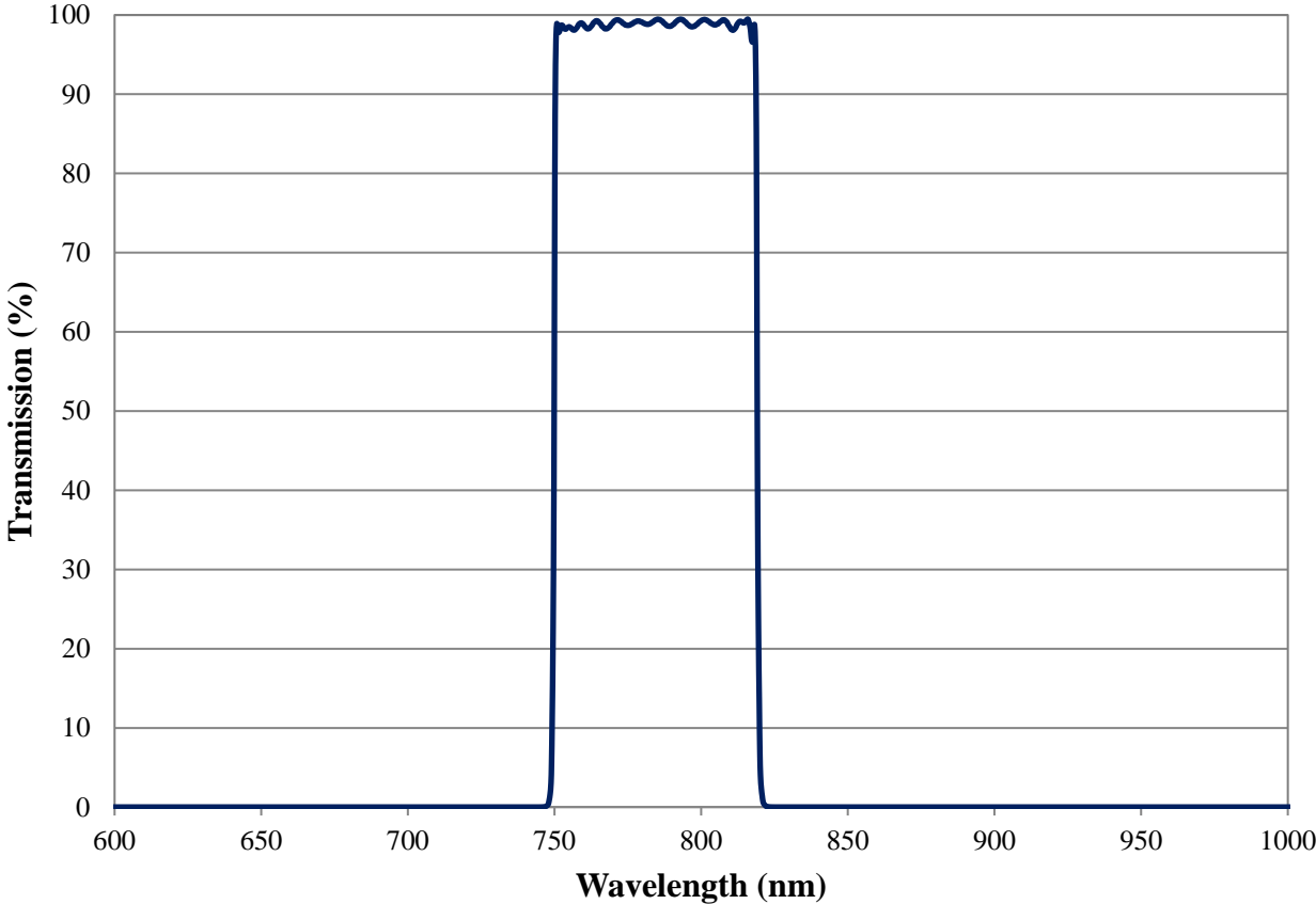
785nm Fluorescence Bandpass Filter: 71nm FWHM OD >6.0 Coating Performance FOR REFERENCE ONLY
