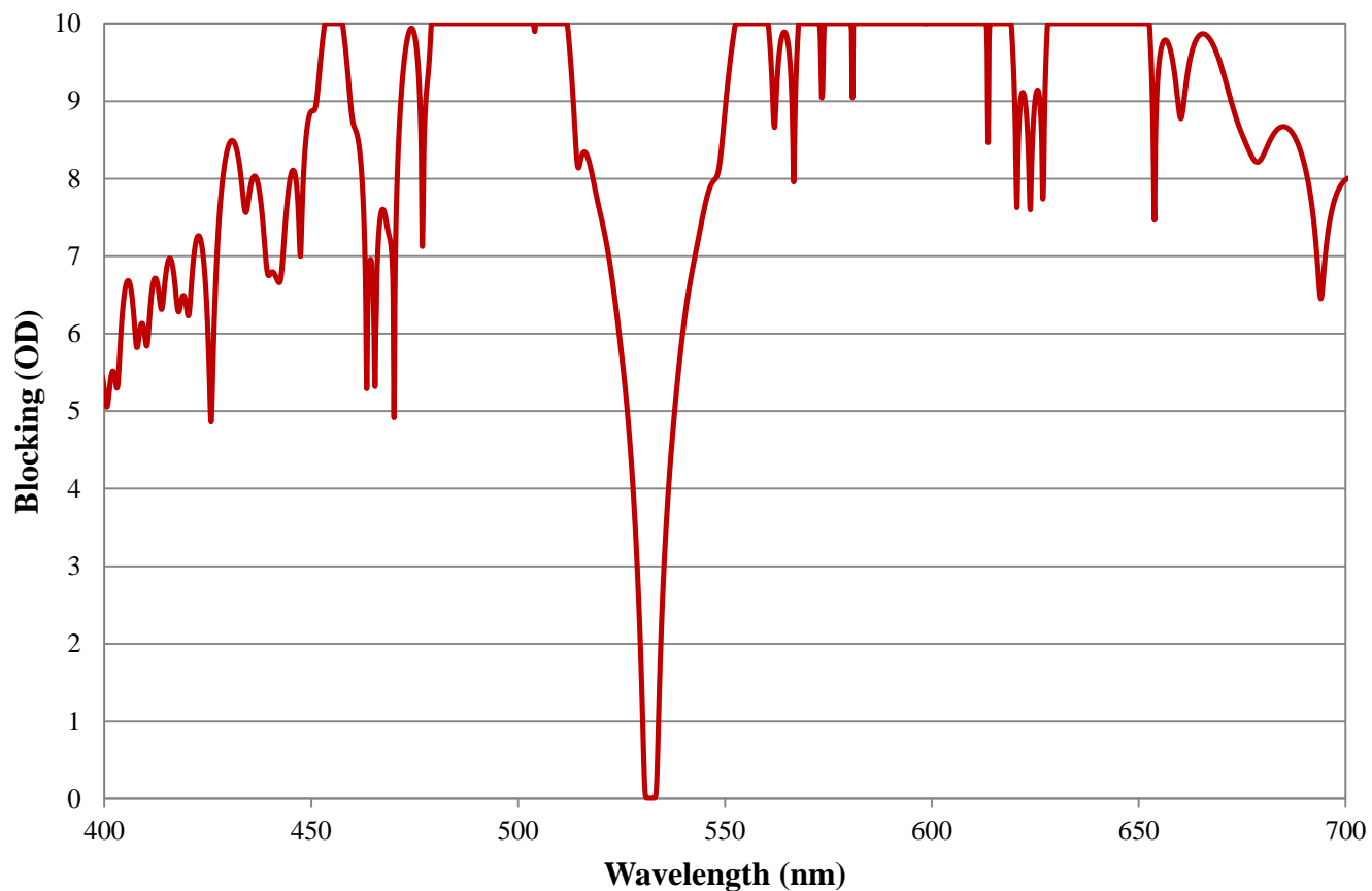
532nm OD 6 Laser-Line Filter, 2.0nm Bandwidth FOR REFERENCE ONLY
